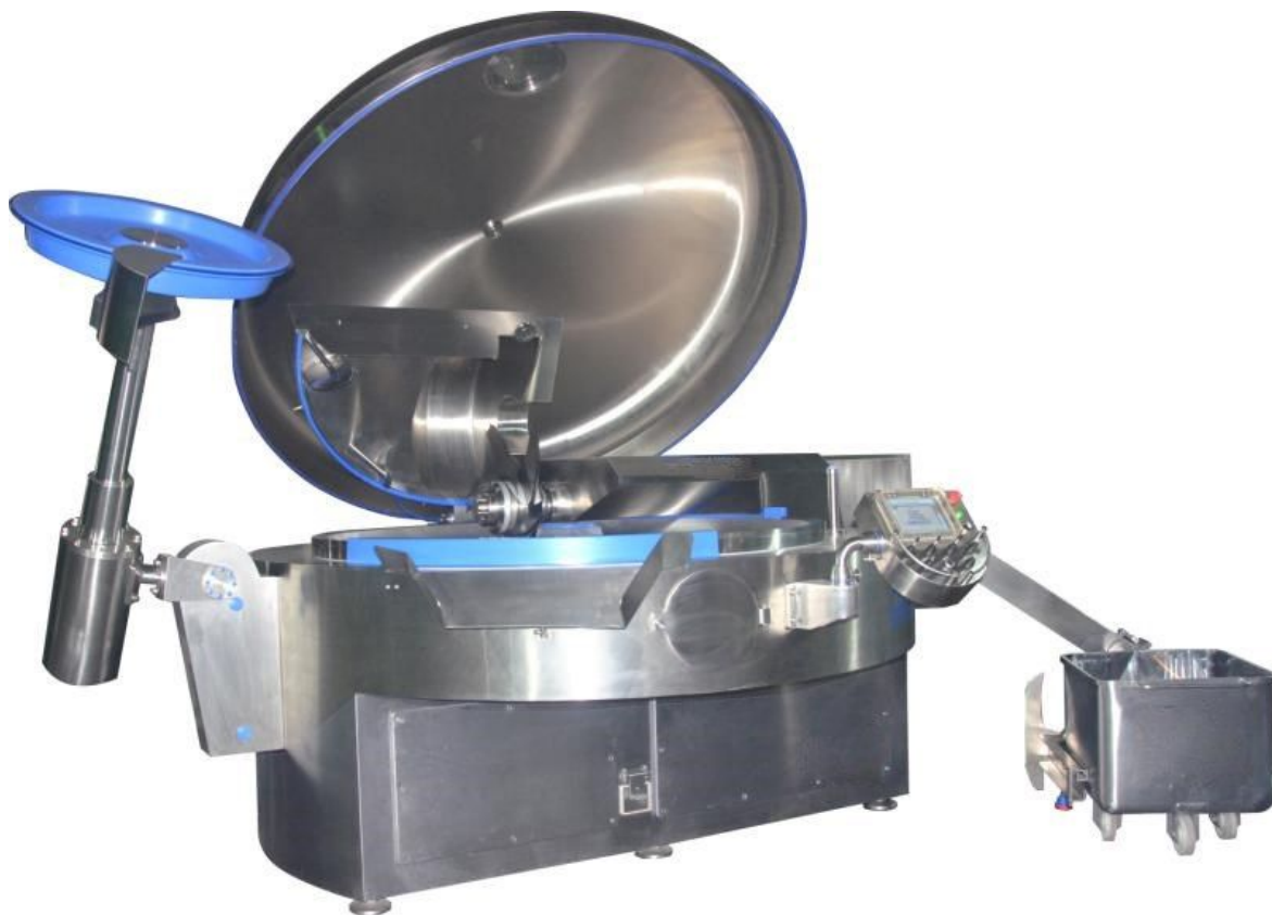
750 Ltr. Vacuum Bowl Cutter with loader
